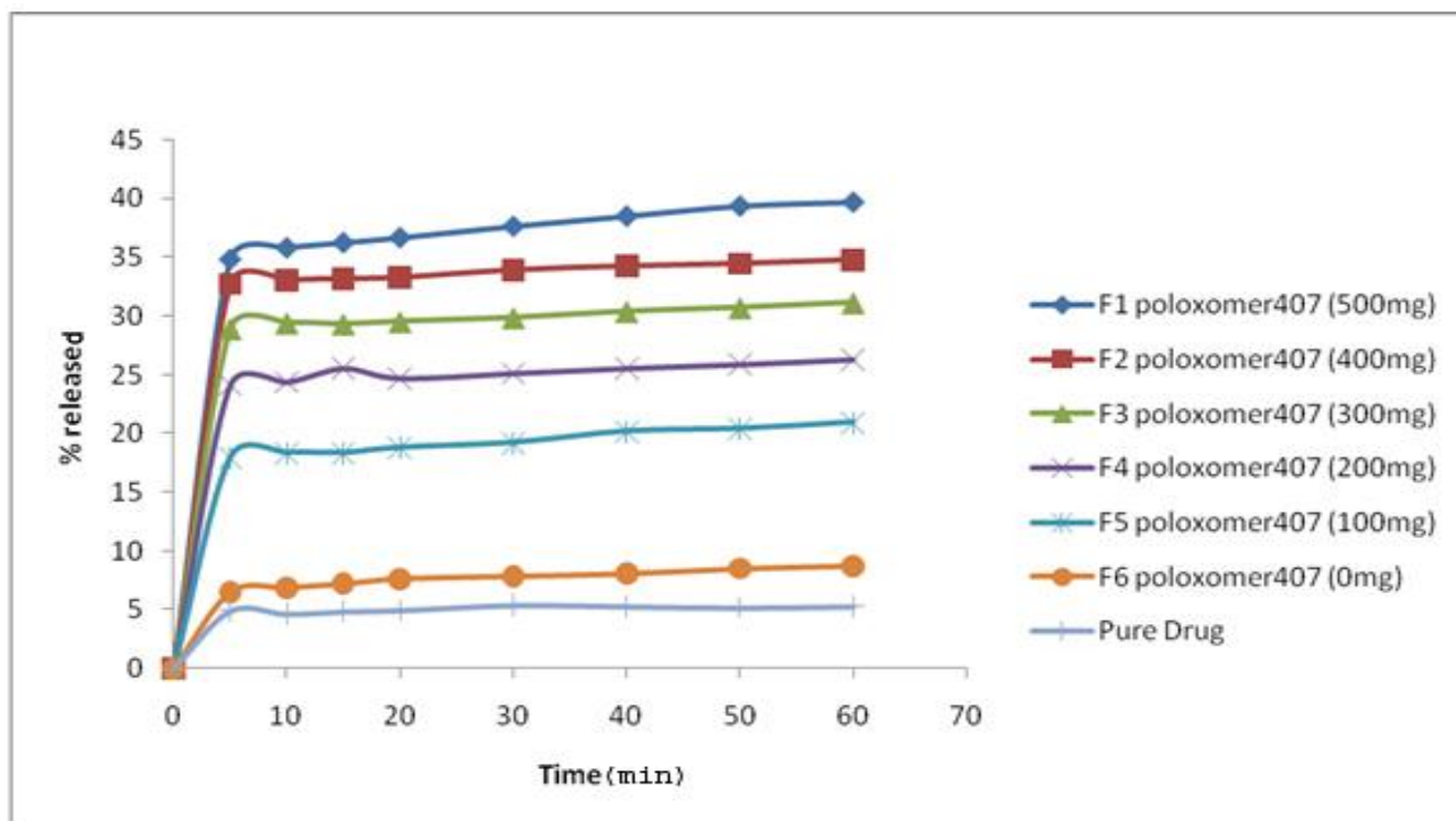
Fig 5. DRUG RELEASE FROM PLOXOMER 407 FORMULATIONS (Error bars were not shown to ensure clarity, n=3)
